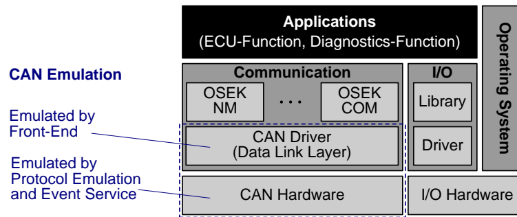
Fig. 8. Model of an Automotive ECU
